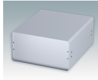
M5504110 UNICASE 4 Aluminium Lichtgrau RAL 7035 261x300x134.5mm
