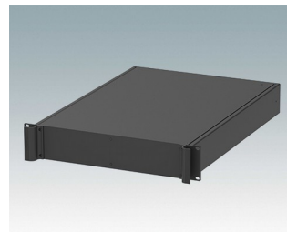
M6219279 COMBIMET 19" 2HEx610mm Aluminium Schwarz RAL 9005 88.1x482.6x609.6mm
