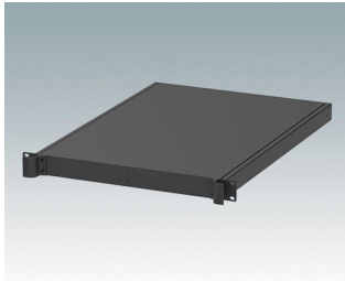
M6219179 COMBIMET 19" 1HEx610mm Aluminium Schwarz RAL 9005 43.6x482.6x609.6mm
