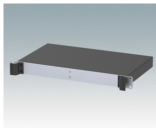
M6219119 COMBIMET 19" 1HEx265mm Solide Oberseite Aluminium Schwarz RAL 9005 43.6x482.6x265mm
